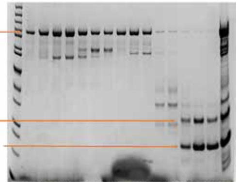
14-07-2020: Gel filtration Mcm6 (Hss) (+Ulp1) (0.7M NaCl+0.025M Tris pH 7.6) prep. (Coomassie Blue). Sample order: Protein ladder, Fractions: 4, 5, 6, 7, 8, 9, 10, 12, 13, 14, 17, 18, 20, 21, 22: Sample after digestion.
